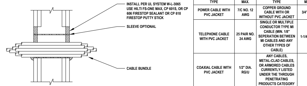
4 CABLE BUNDLE THROUGH GYPSUM WALL ASSEMBLY (2-HR.) E.4.3 NOT TO SCALE
