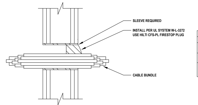
5 CABLE BUNDLE THROUGH GYPSUM WALL ASSEMBLY (2-HR.) E.4.3 NOT TO SCALE
