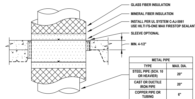
4 M.3.3 METAL PIPE WITH GLASS FIBER INSULATION THROUGH CONCRETE OVER METAL DECKING (3-HR.) NOT TO SCALE
